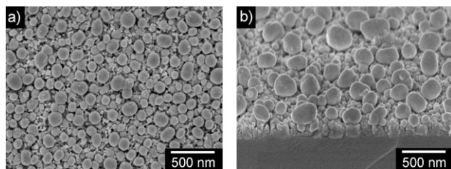
Figure 1. Typical SEM images of tungsten oxide films deposited from the electrolyte at a pH of about 8.6: a) top view; b) side view from 45°. The morphology of the nanostructures resembles a pebble beach.
